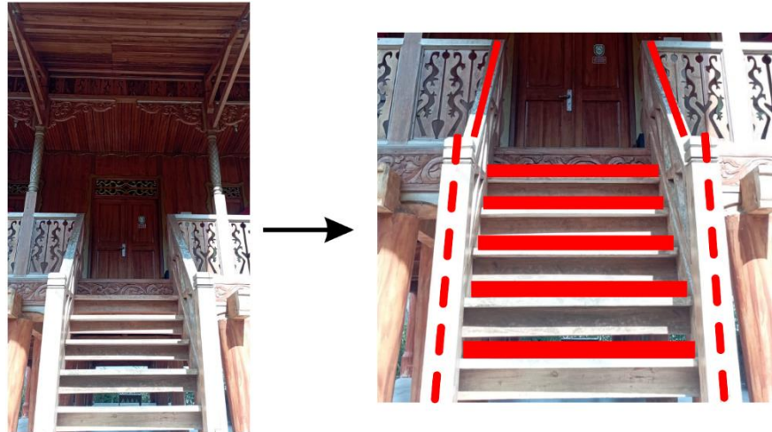
Figure 9. Parallel Lines
