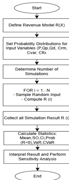
Figure 2. Monte Carlo Simulation
