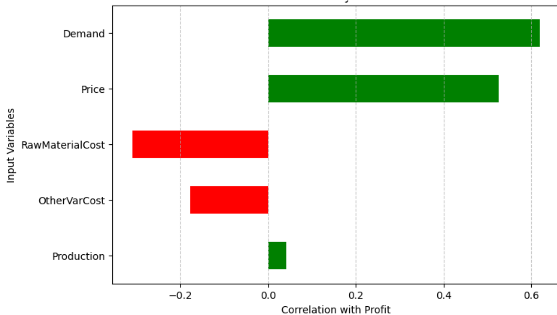
Figure 4. Sensitivity of Variables on Profit
