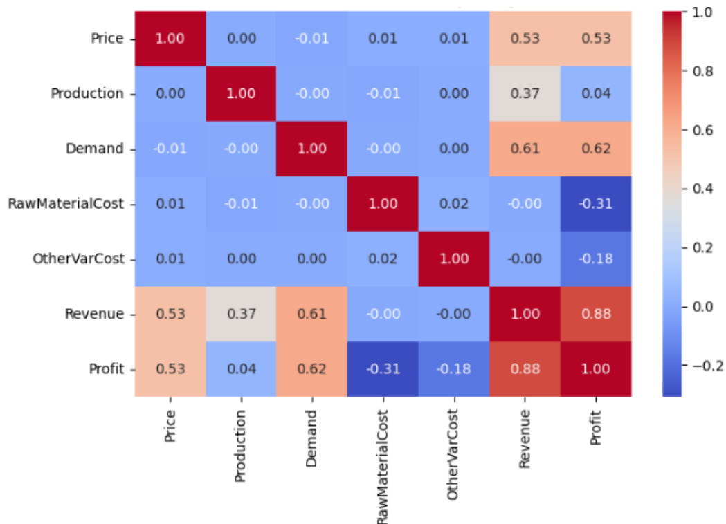
Figure 5. Correlation Matrix
