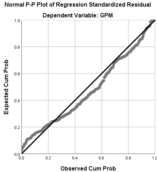
Figure 1. Normal P P Plot of Residuals
