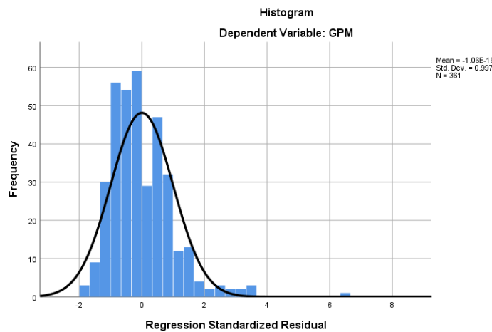
Figure 2. Normal Histogram of Residuals
