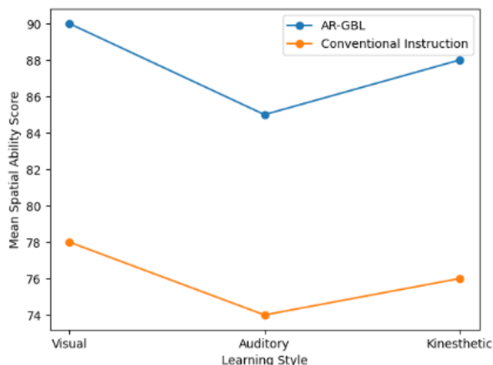
Figure 1. Interaction Plot
