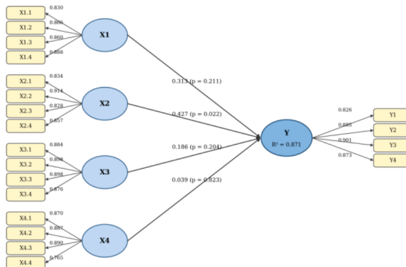
Figure 2. Estimated measurement and structural model
