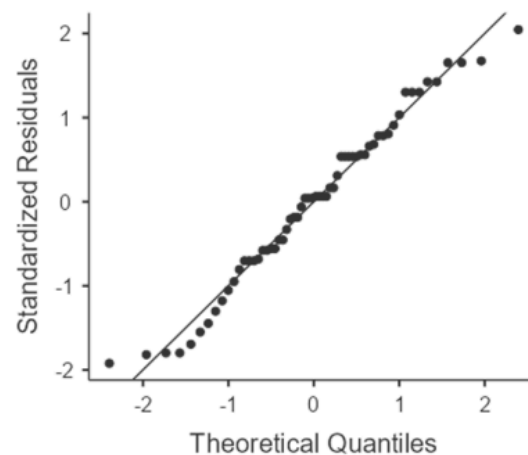
Figure 2. Quantile-Quantile (Q-Q) Plot for Normality Assessment
