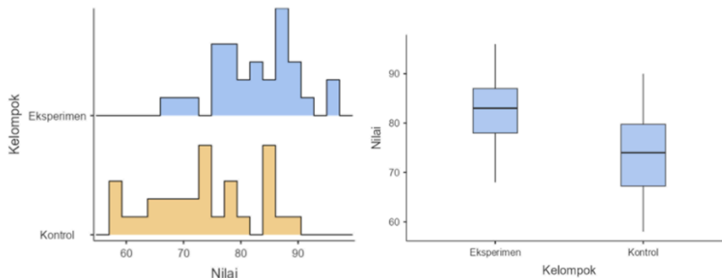
Figure 1. Distribution Plots and Comparative Visualization
