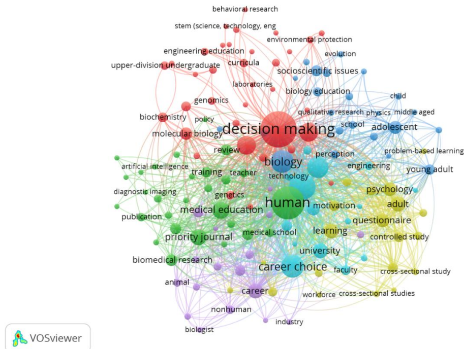
Figure 4. Network Visualization
